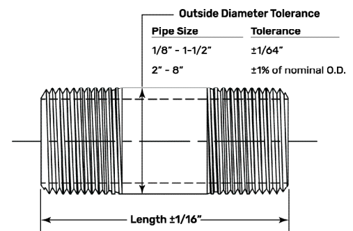
Nipples over 12" long have a length tolerance of \pm 1/8" .
